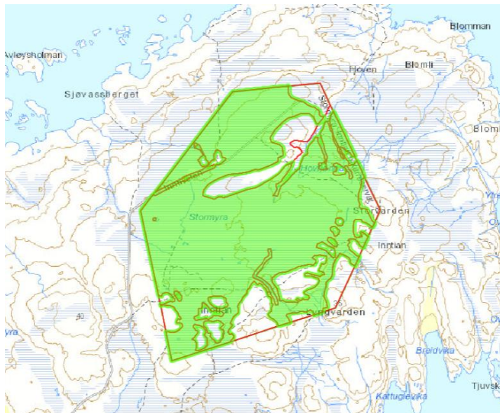
Fig 2. Naturtypekartlegging. Naturbase
